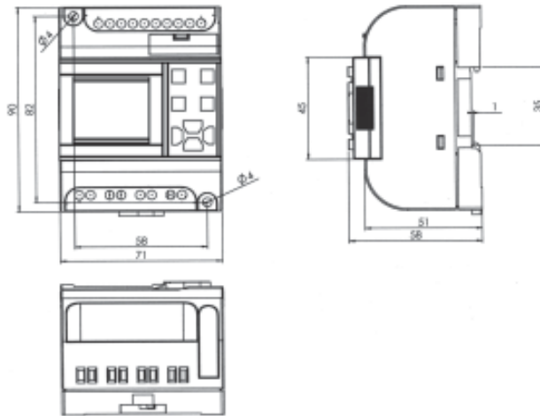
Fig 2.3 FAB-10 Series installation dimensions (Unit: mm)
