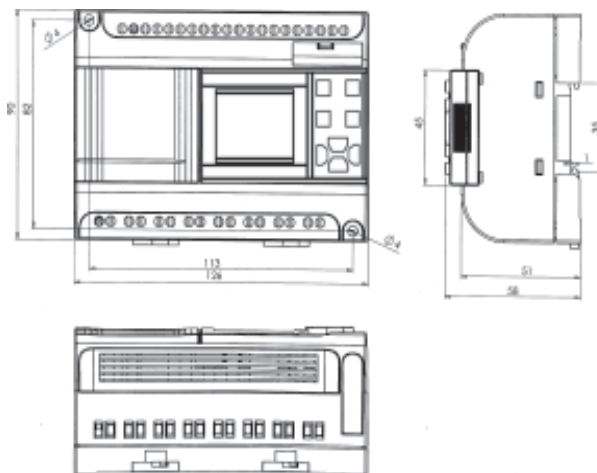
Fig 2.3 FAB-20 Series installation dimensions (Unit: mm)
