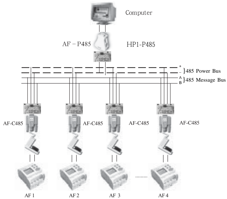
Fig. 2.12 Connecting method
