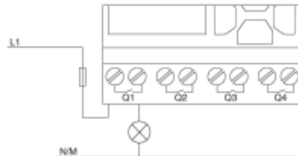
Fig 2.10 Relay Output
