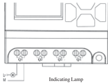
Fig. 2.1 Transistor Output
