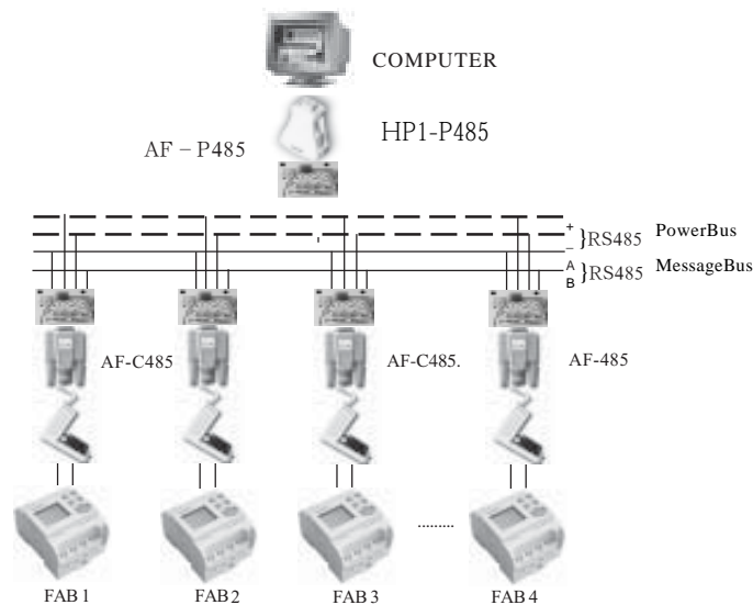
Fig. 1-1 Serial Communication Using RS485
