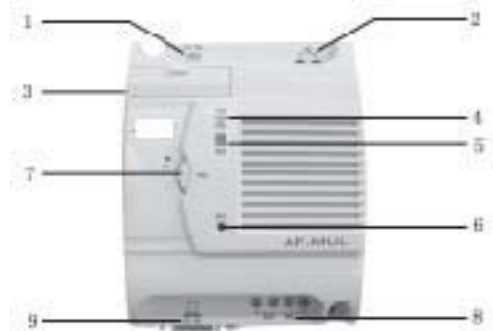
Fig 6.1 Structure of AF-MUL
