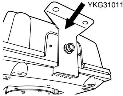
YKG31011, Flat angle bracket for luxlift 12kg type (2 pcs./set)
