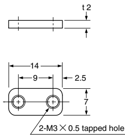
MS-GXL15 Sensor mounting bracket for GXL-15 type (Optional)
