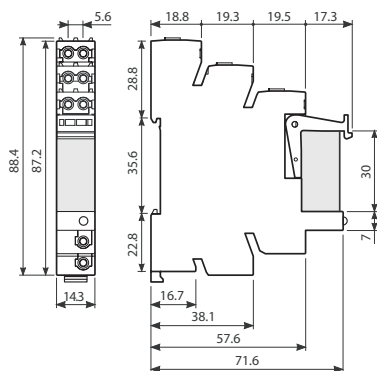
Dimensioni in mm Dimensions in mm
