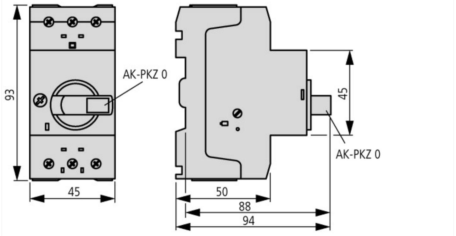
Motor-protective circuit-breakers with lockable rotary handles PKZM0-...+AK-PKZ0
