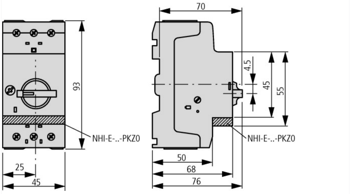
Motor-protective circuit-breaker with standard auxiliary contact PKZM0-...(+NHI-E-...-PKZ0) PKZM0-...-T(+NHI-E-...-PKZ0) PKM0-...(+NHI-E-...-PKZ0)
