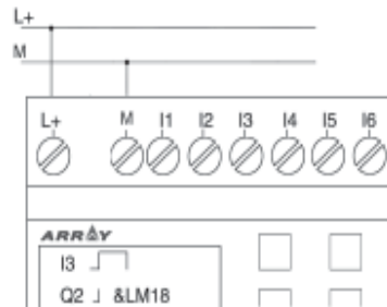
Fig 2.8 DC Type ( E Type)
