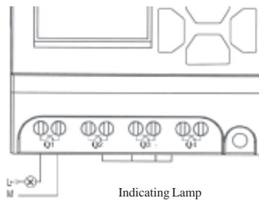
Fig. 2.1 Transistor Output
