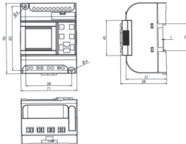
Fig 2.3 AF-10 FAB Series installation dimensions (Unit: mm)
