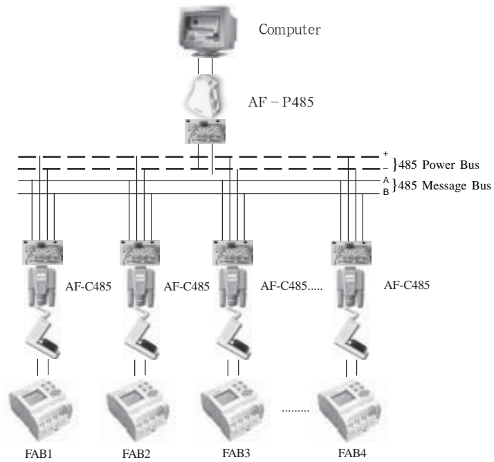
Fig. 2.12 Connecting method
