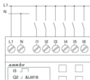
Fig 2.7 AC Type
